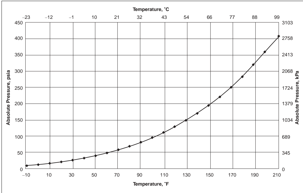
Figure 1. Saturated Vapor Pressure of DuPont™ FE-227™
